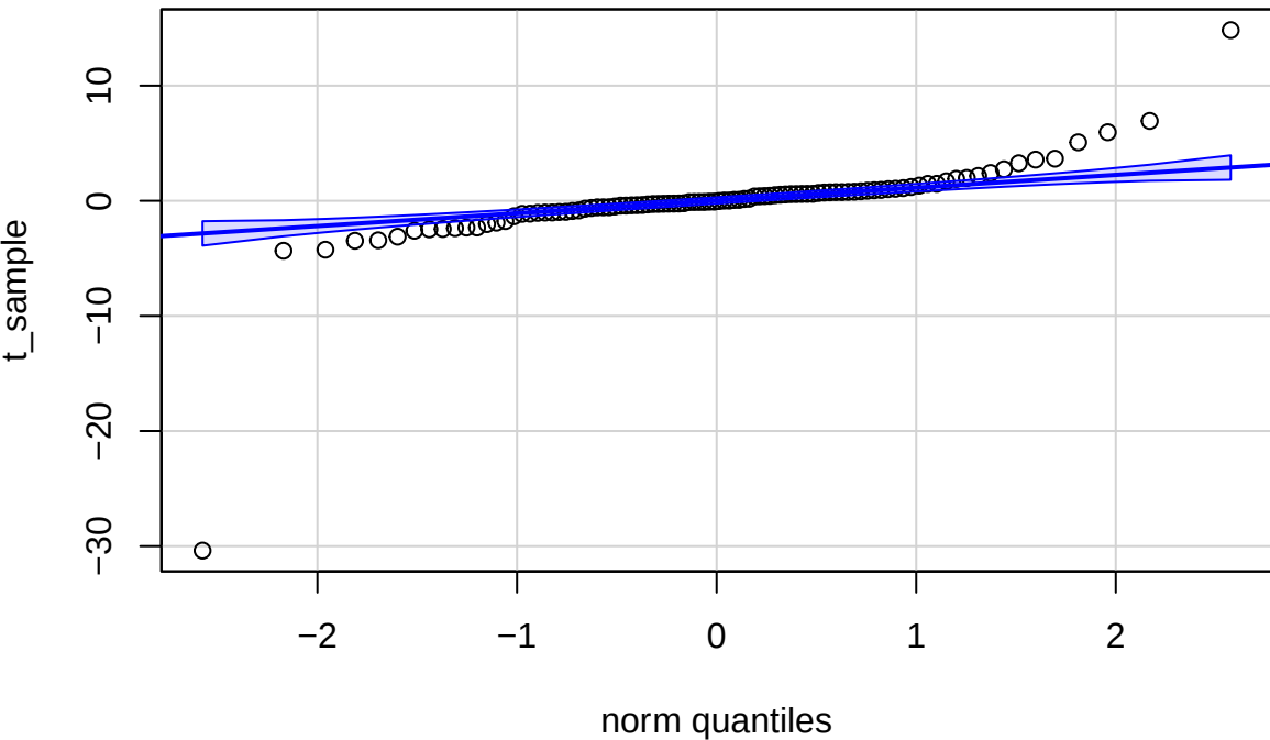
Q-Q Plot: t-Distribution vs Normal
