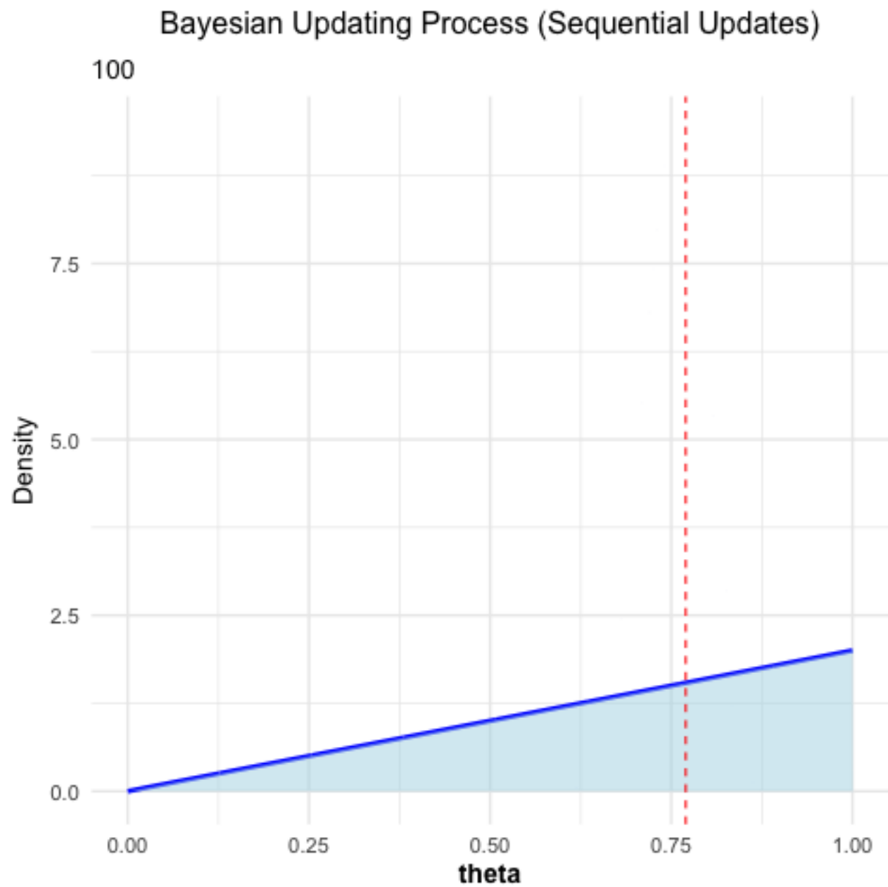
Figure 3.1: Bayesian updating: the posterior converges towards the true value as more coin tosses are observed.
