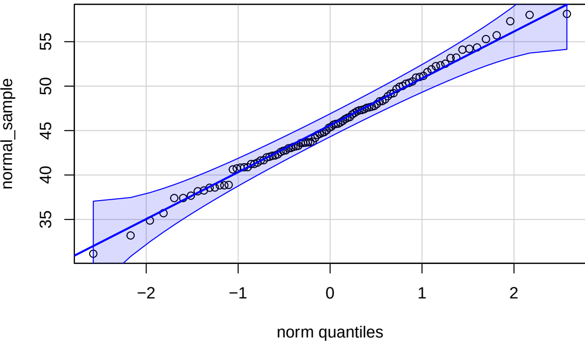
Q-Q Plot: Normal Distribution
