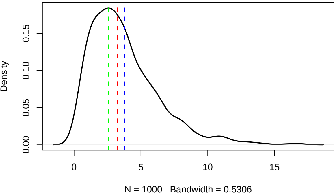
Density Curve with Mean, Median, and Mode
