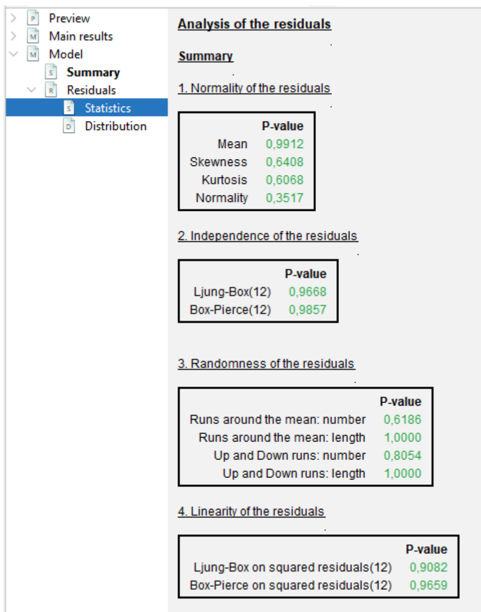
Figure 115: Tests on the residuals of the Regression Model
