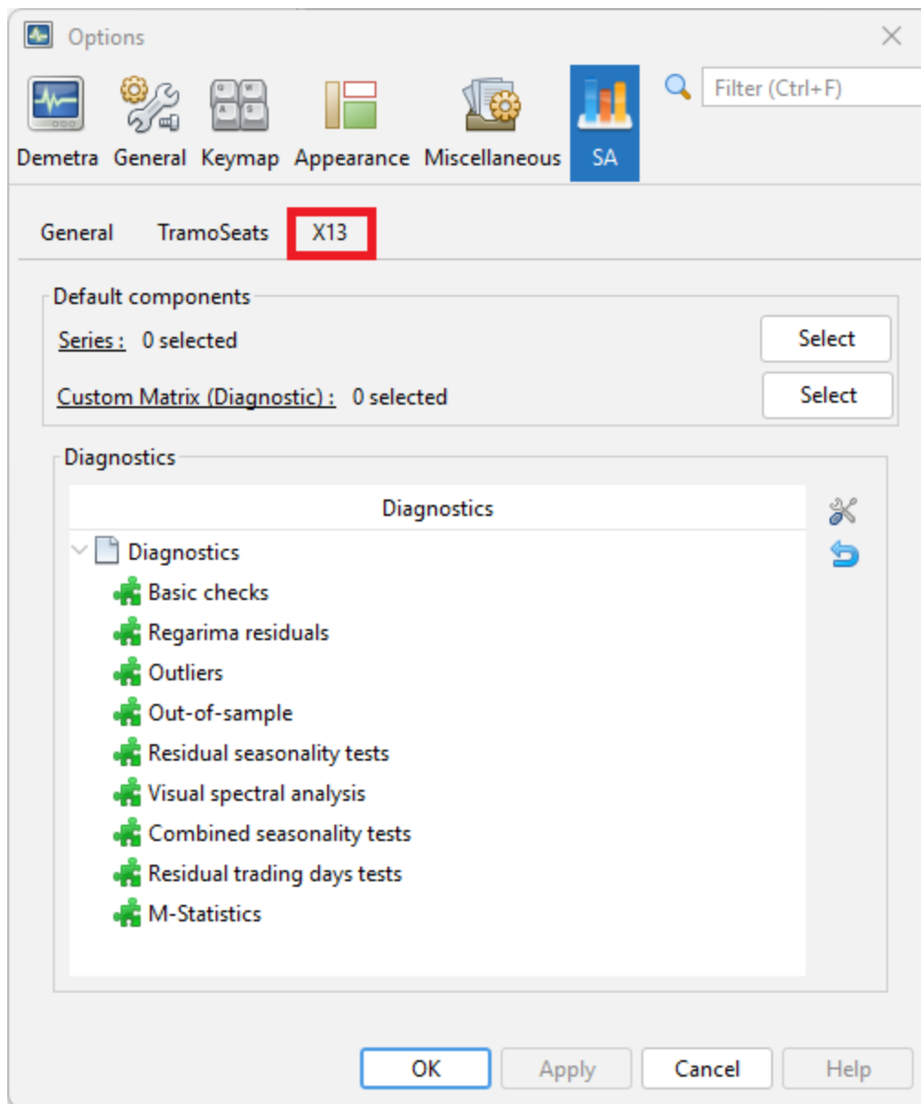
Figure 187: Settings for the quality measures and tests in X-13 in v3
