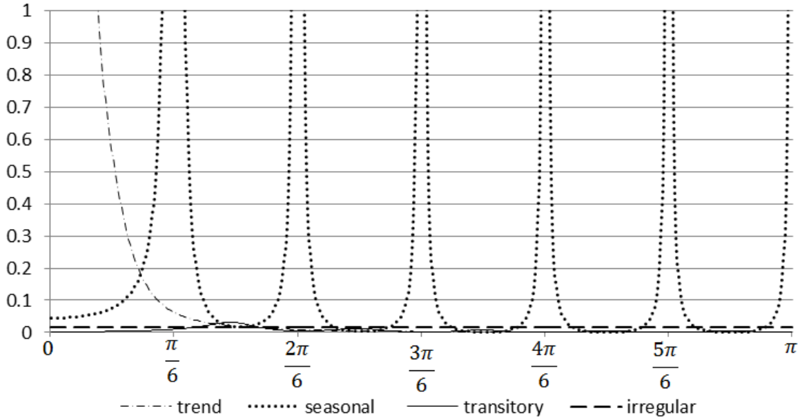
Figure 279: The pseudo-spectra for the components
