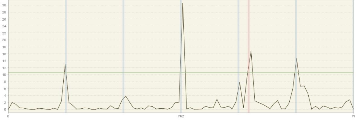
Figure 267: Periodogram with seasonal (grey) and calendar (red) frequencies highlighted
