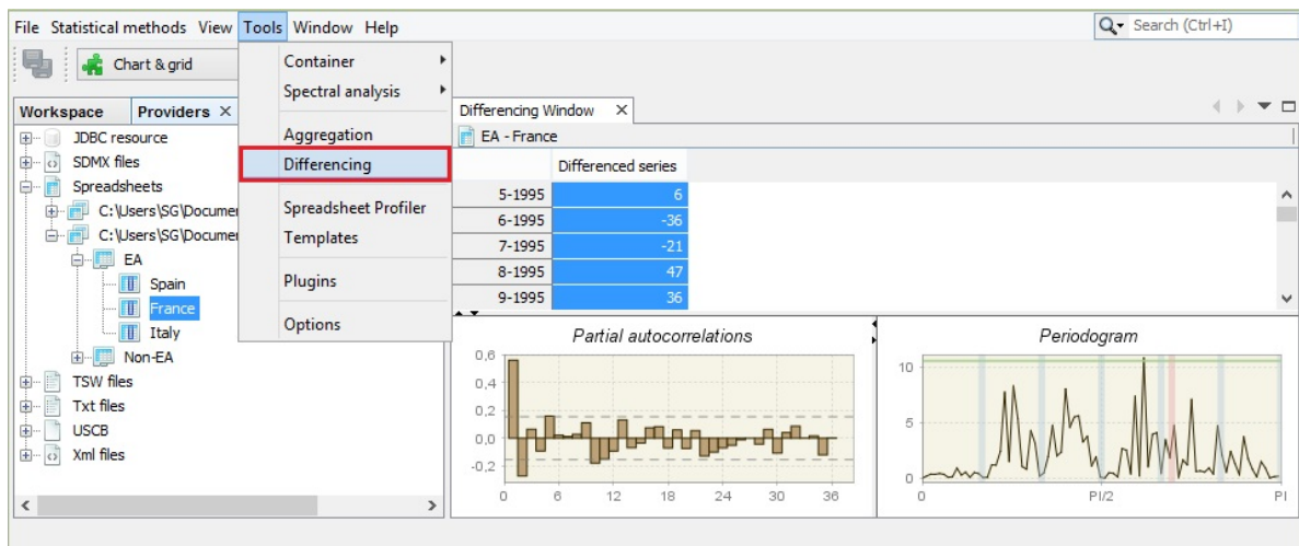
Figure 221: The *Differencing tool
