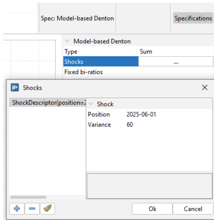
Figure 118: Model-based Denton Specifications (Shocks)
