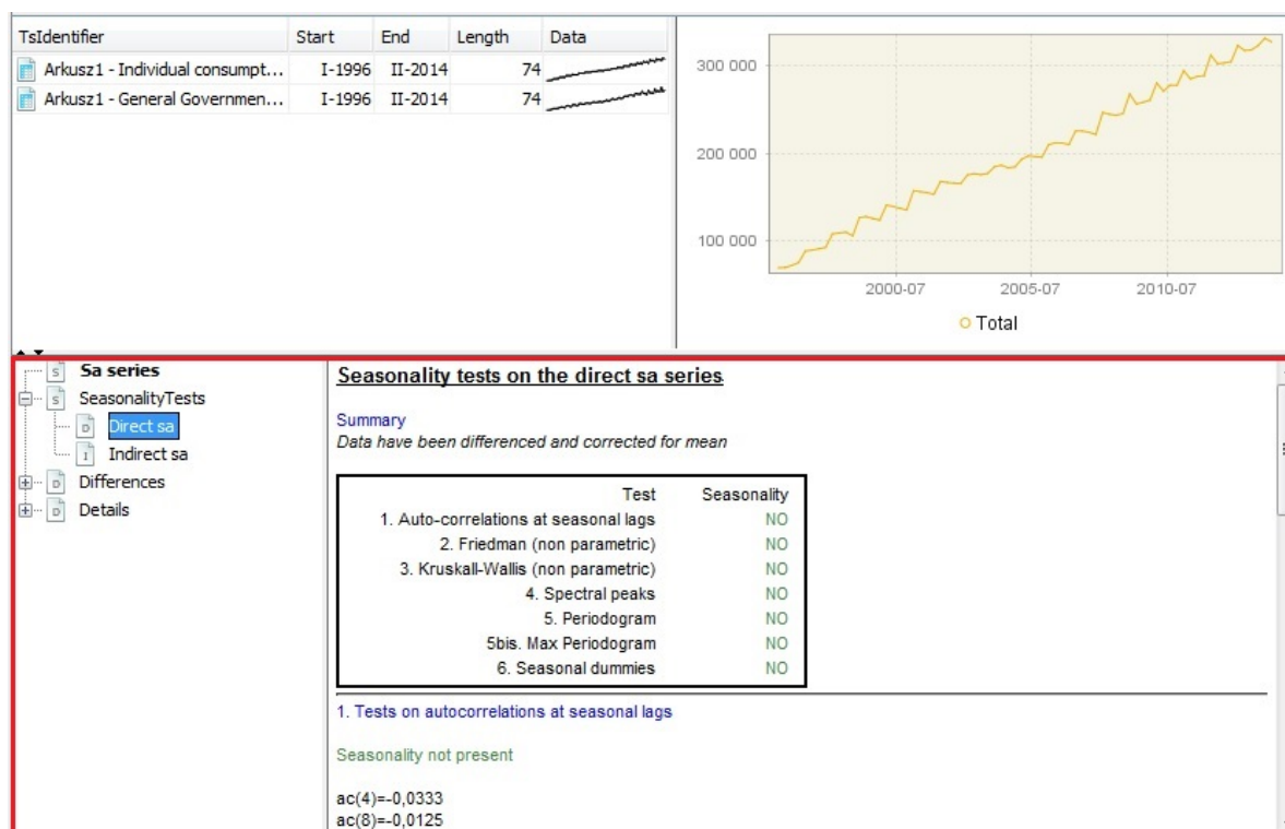
Figure 241: Seasonality tests' results for a direct seasonal adjustment
