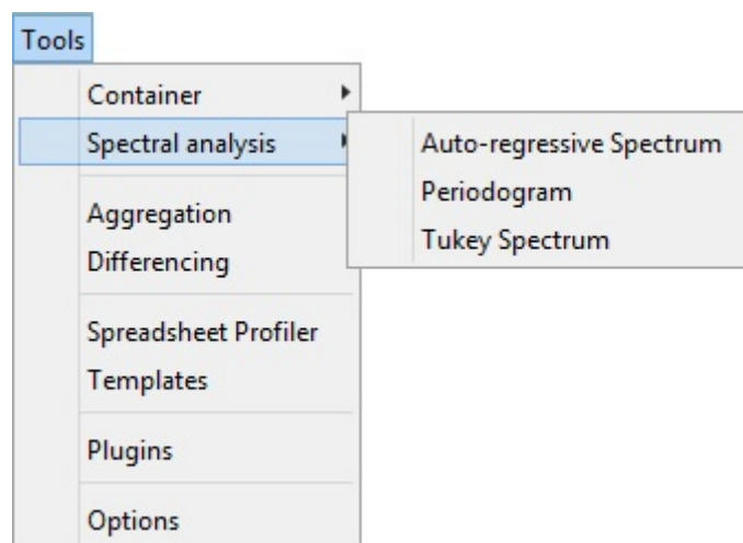
Figure 149: Tools for spectral analysis
