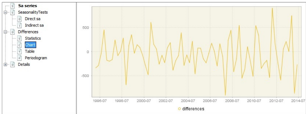
Figure 242: Graph presenting the differences between direct and indirect seasonal adjustment results
