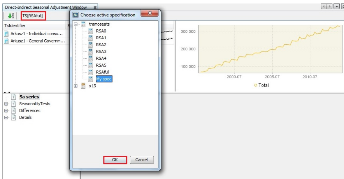
Figure 239: Choosing a specification for the analysis
