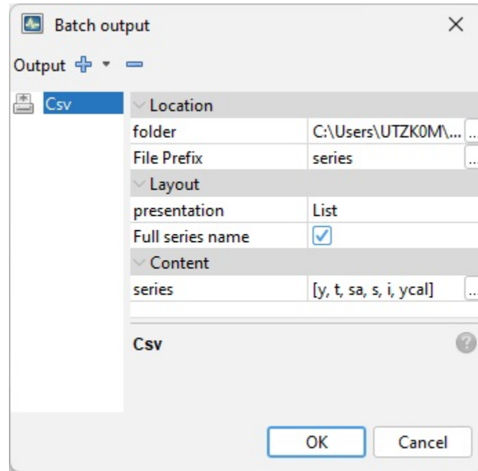
Figure 244: Options for a .csv format
