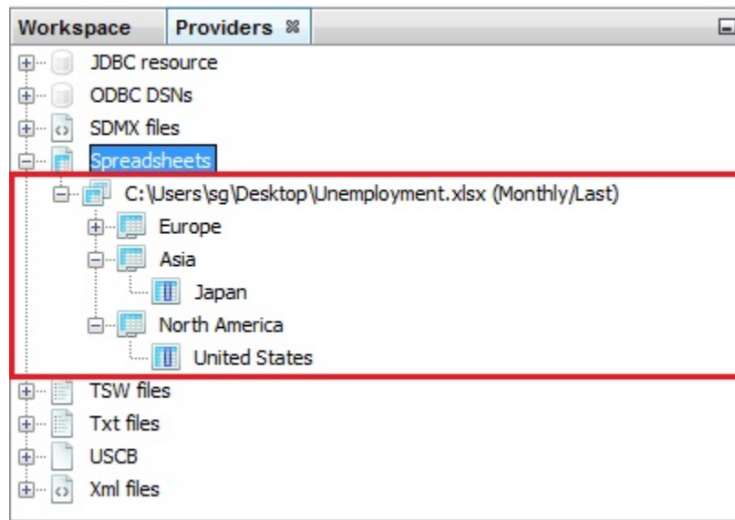
Figure 128: A structure of a dataset
