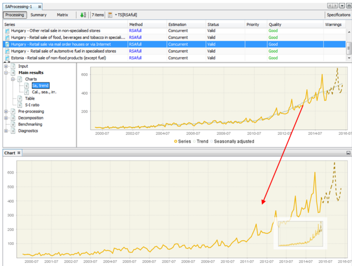
Figure 203: Displaying the seasonally adjusted series on a separate chart
