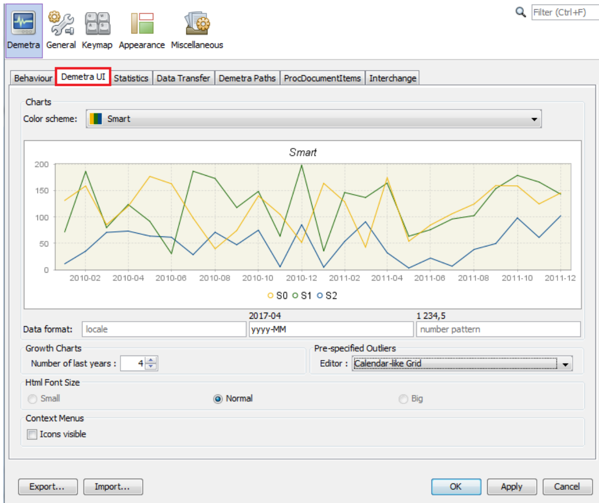
Figure 164: The content of the Demetra UI tab
