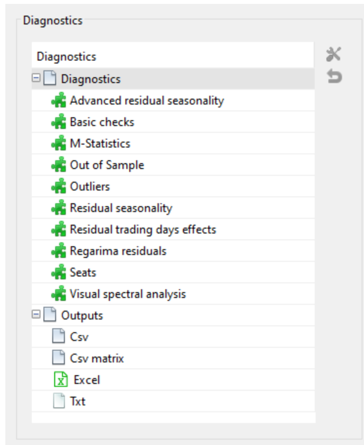
Figure 185: The Diagnostics section in v2
