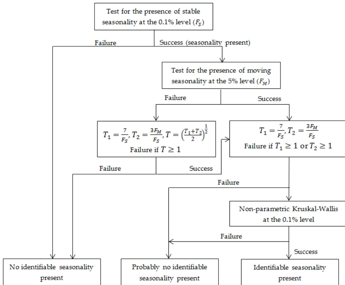
Figure 287: Combined seasonality test , source: LADIRAY, D., QUEN-NEVILLE, B. (2001)
