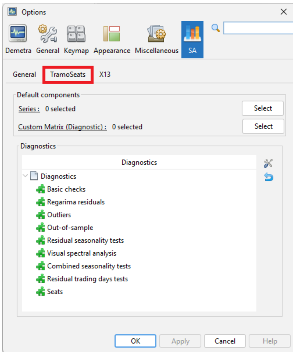
Figure 183: Settings for the quality measures and tests in TramoSeats in v3
