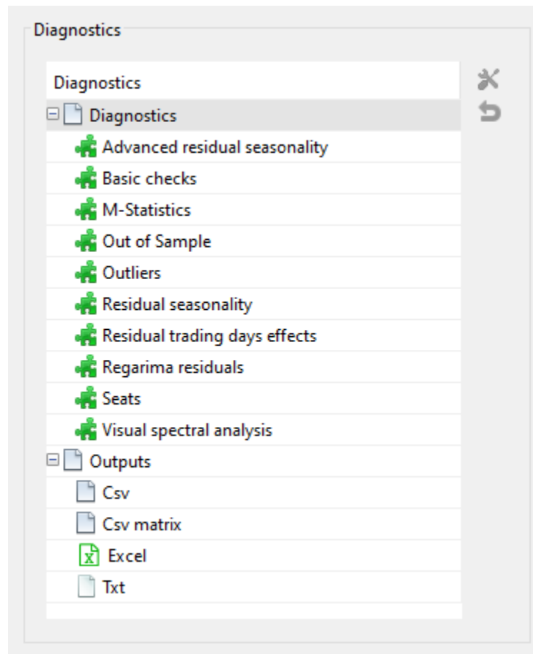
Figure 182: The Diagnostics section in v2
