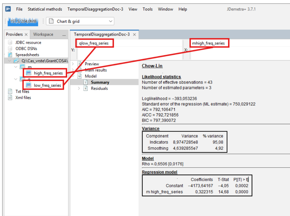
Figure 112: Temporal Disaggregation procedure
