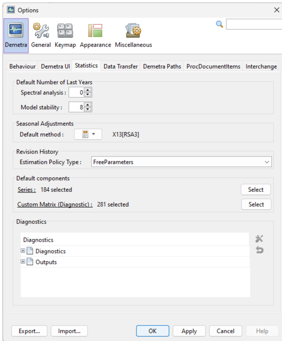
Figure 175: Statistics tab in v2
