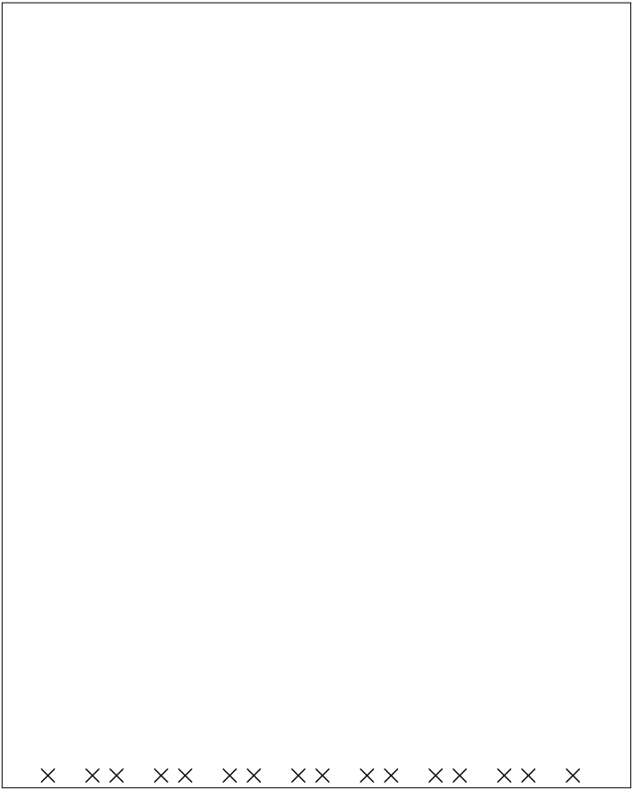
Drill Map: X 2.476mm / 0.0975" (16 holes) (not plated)
