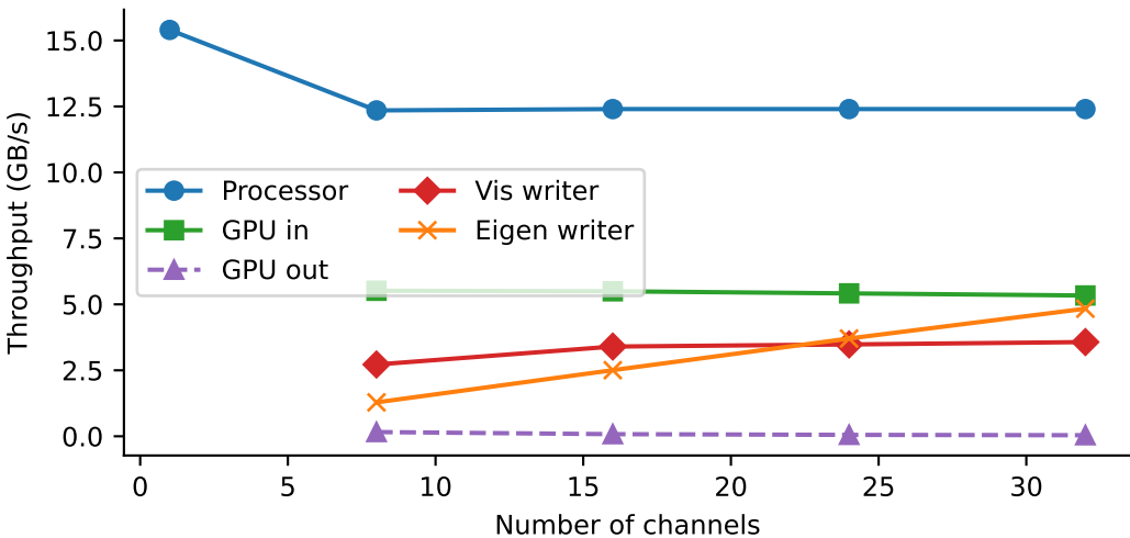
Pipeline stage throughput comparison
