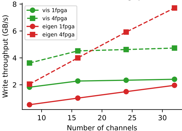
HDF5 writer throughput
