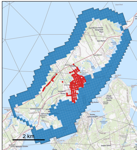
A. Coarse, 6,491 cells
