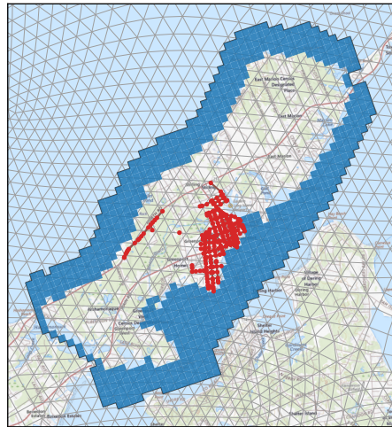
C. Fine, 41,091 cells
