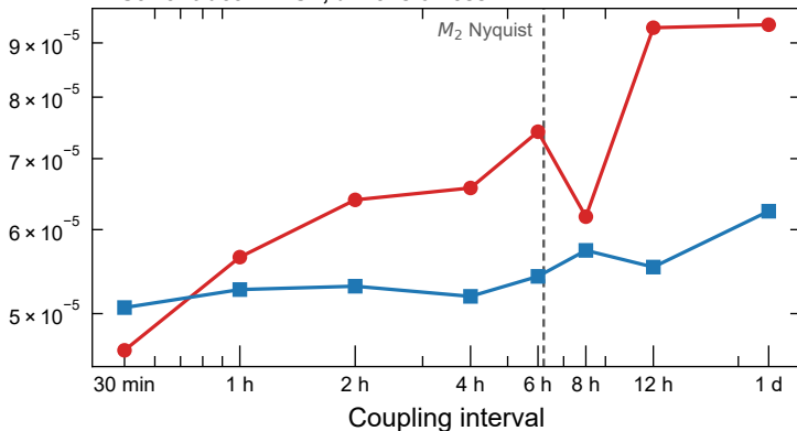
C. Sewer tracer RMSE, dimensionless
