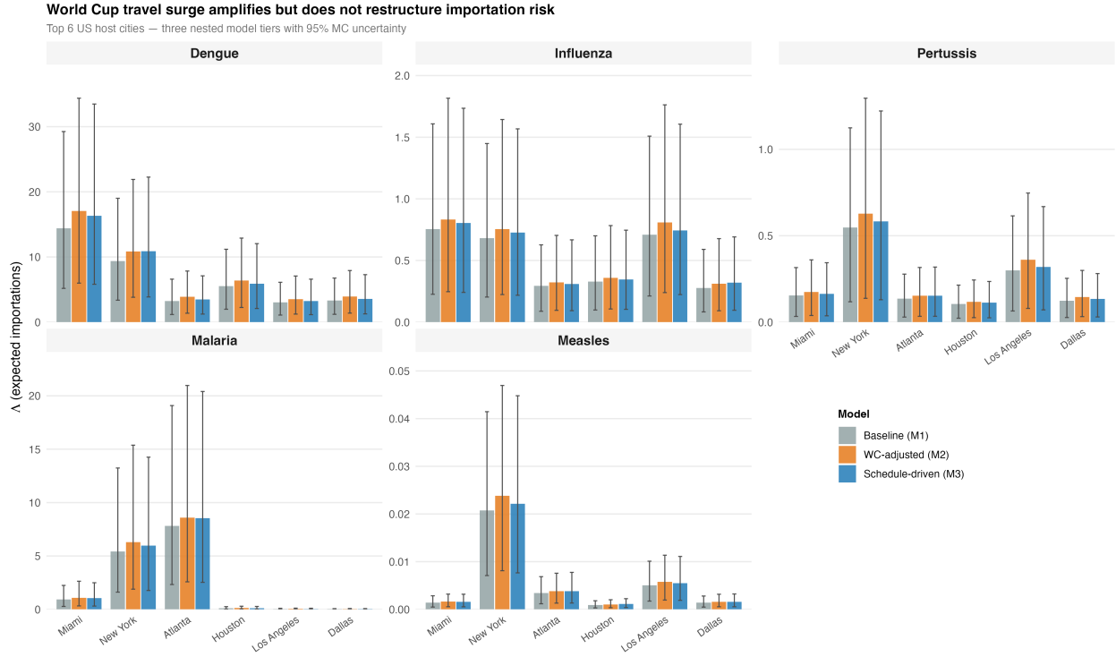
Figure 3: Three-model comparison of expected importations ( \Lambda ) for the six highest-risk US venue cities. Each panel shows one disease; bars are grouped by city and filled by model tier: Baseline (Model 1, routine June 2024 travel), WC-adjusted (Model 2, June 2026 projections), and Schedule-driven (Model 3, fan routing by match schedule). Bars show the MC median; whiskers span the 95% uncertainty interval (5,000 Uniform draws on \rho_d and p_d ). The step-up from Model 1 to Model 2 is near-uniform across cities, confirming that the World Cup surge amplifies risk proportionally. The further step from Model 2 to Model 3 produces city-specific divergence driven by schedule-based redistribution toward match venues.
