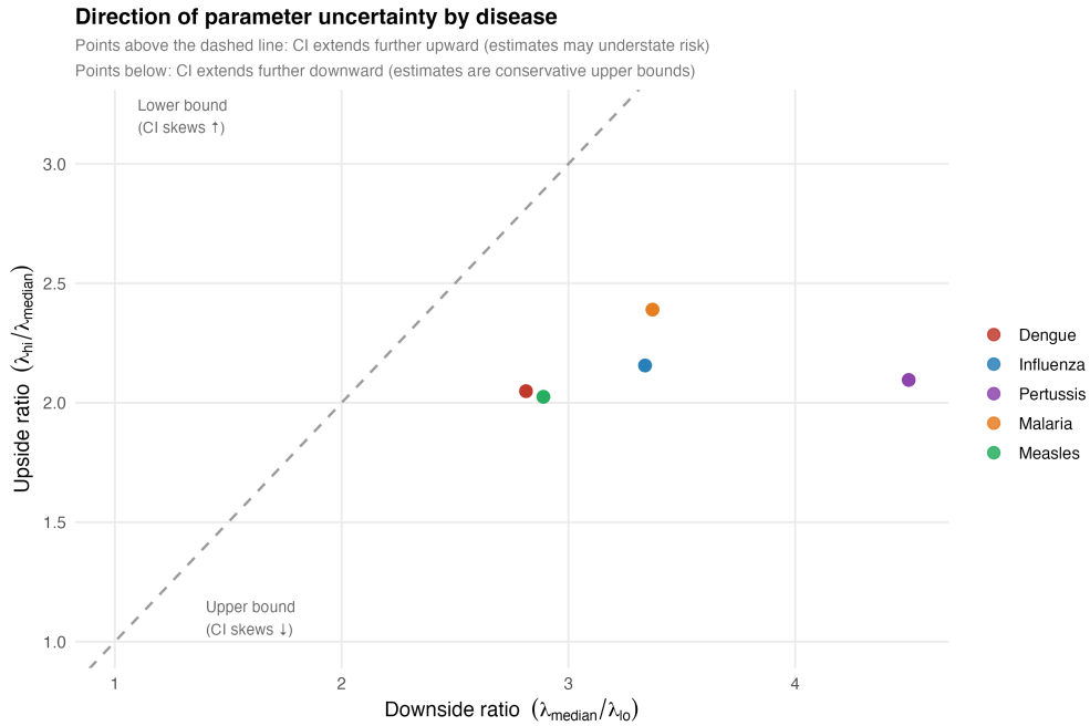
Figure 6: Direction of Monte Carlo parameter uncertainty by disease. Each point represents one disease–city pair under the schedule-driven model. Upside ratio = \Lambda_{hi}/\Lambda_{median} ; downside ratio = \Lambda_{median}/\Lambda_{lo} . Points above the dashed diagonal: CI skews upward (central estimate near lower bound of plausible range). Points below: CI skews downward (central estimate near upper bound). Dengue and influenza may be underestimated; pertussis estimates are conservative upper bounds.
