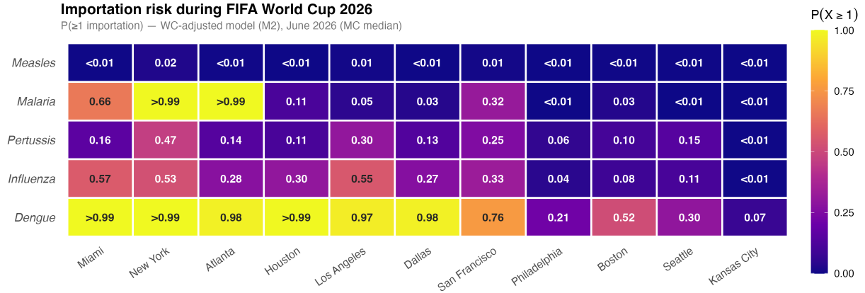
Figure 8: Importation risk overview under the WC-adjusted model (Model 2): P(\geq 1 \text{ importation}) using June 2026 projected arrivals scaled by NTTD growth factors (MC median, 5,000 draws). Same city and disease ordering as Figure 1.
