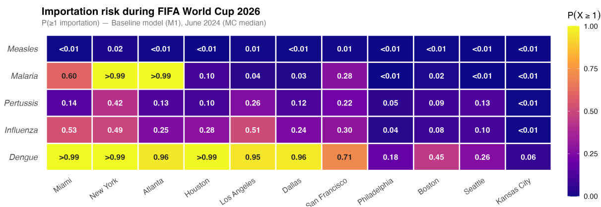
Figure 7: Importation risk overview under the Baseline model (Model 1): P(\geq 1 \text{ importation}) using routine June 2024 COR arrivals with no World Cup growth adjustment (MC median, 5,000 draws). Same city and disease ordering as Figure 1.
