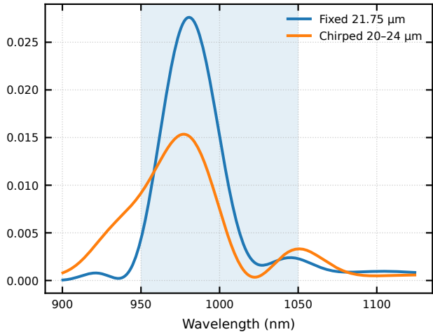
Pump GDD = 0 \text{ fs}^2
