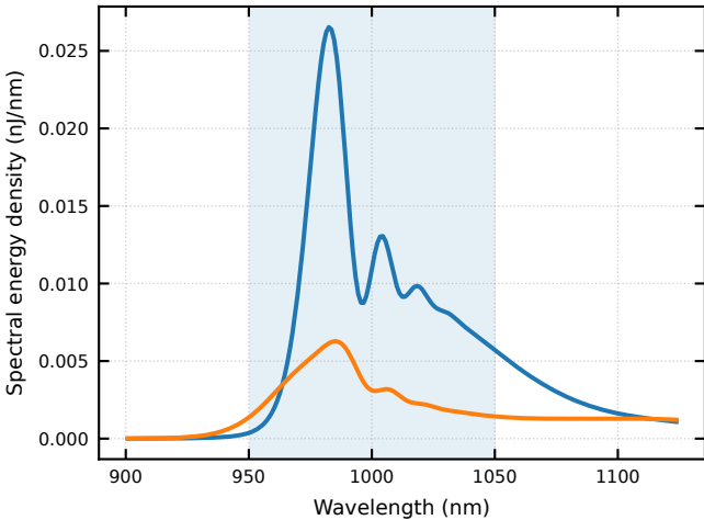
Pump GDD = -1230 \text{ fs}^2
