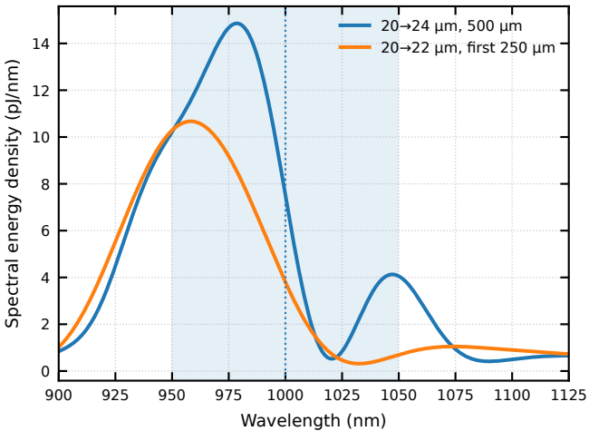
Increasing chirp
