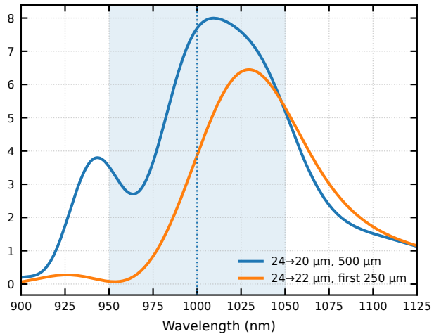
Decreasing chirp
