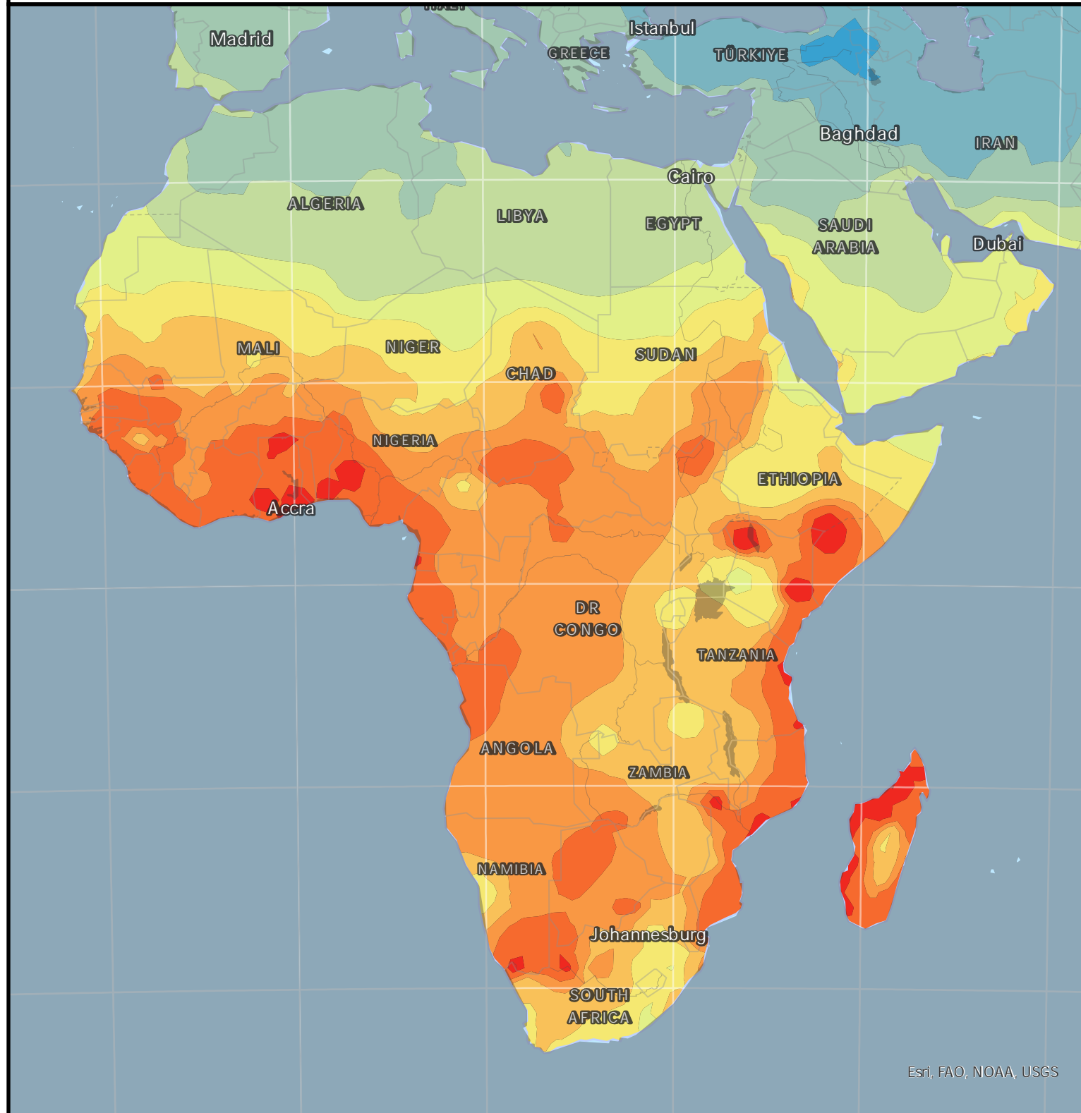
IDW (Inverse Distance Weighted)
