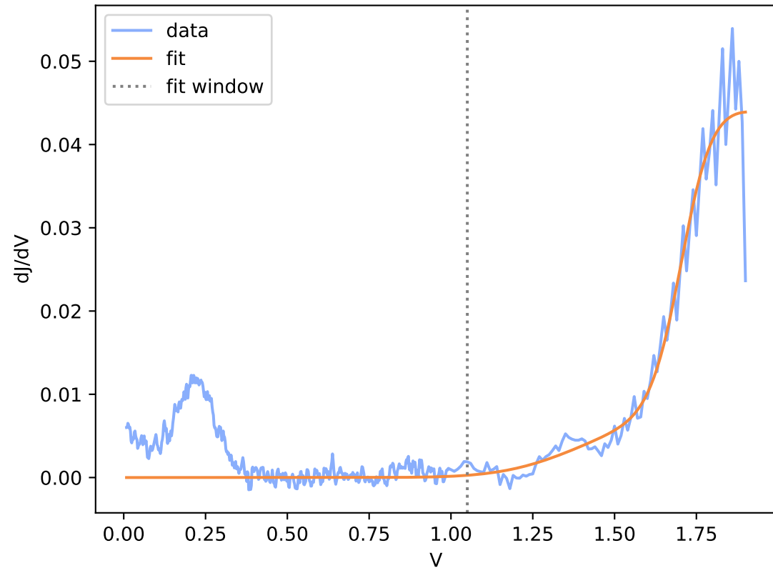
Run10-2-spot30.DTA.csv (window R^2 = 0.956 )
