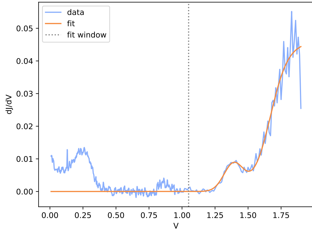
Run10-2-spot39.DTA.csv (window R^2 = 0.952 )
