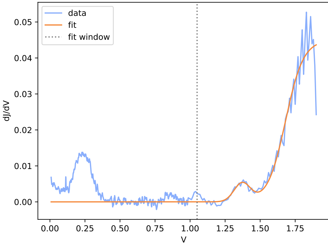
Run10-2-spot44.DTA.csv (window R^2 = 0.953 )
