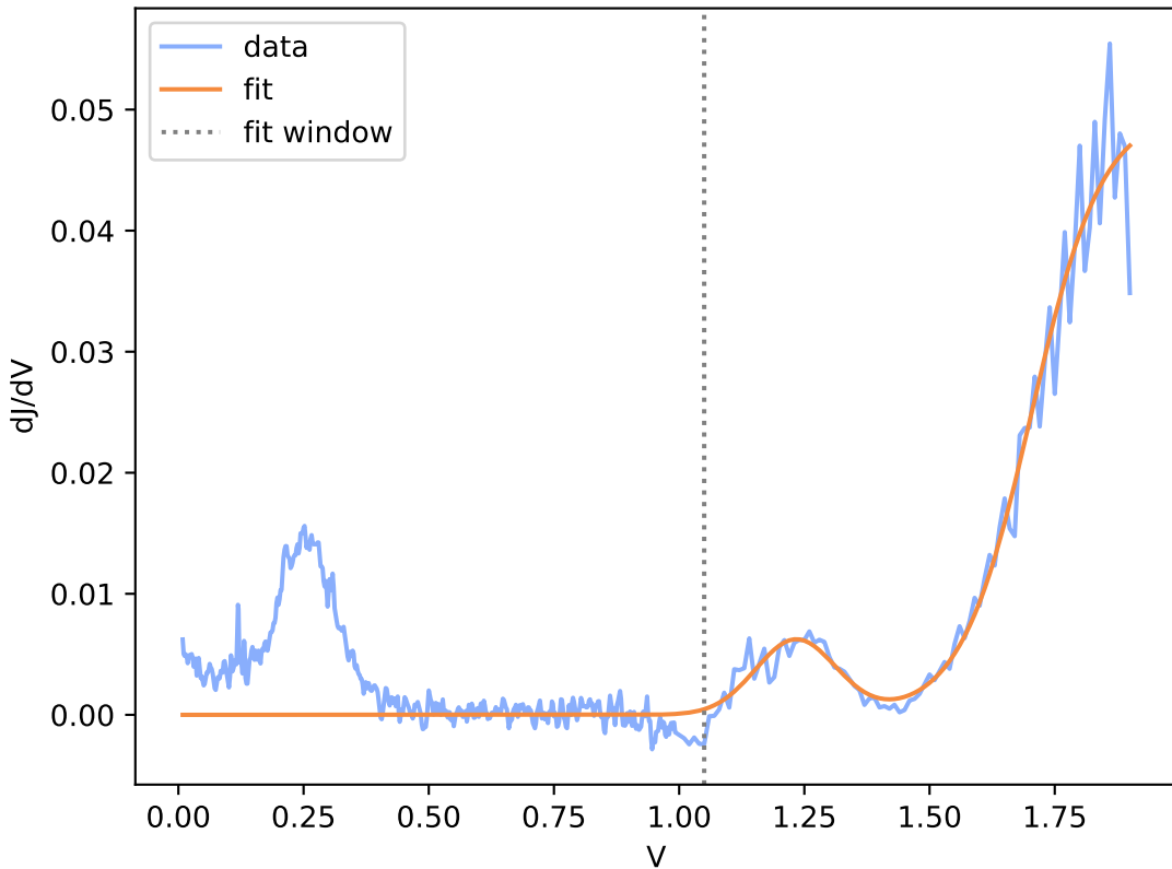
Run10-2-spot6.DTA.csv (window R^2 = 0.970 )
