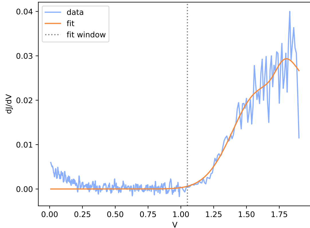
Run12-spot41.DTA.csv (window R^2 = 0.882 )
