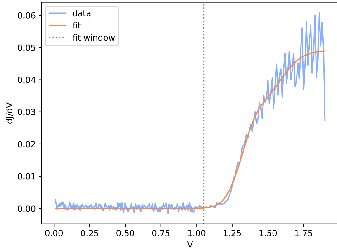
Run12-spot44.DTA.csv (window R^2 = 0.937 )
