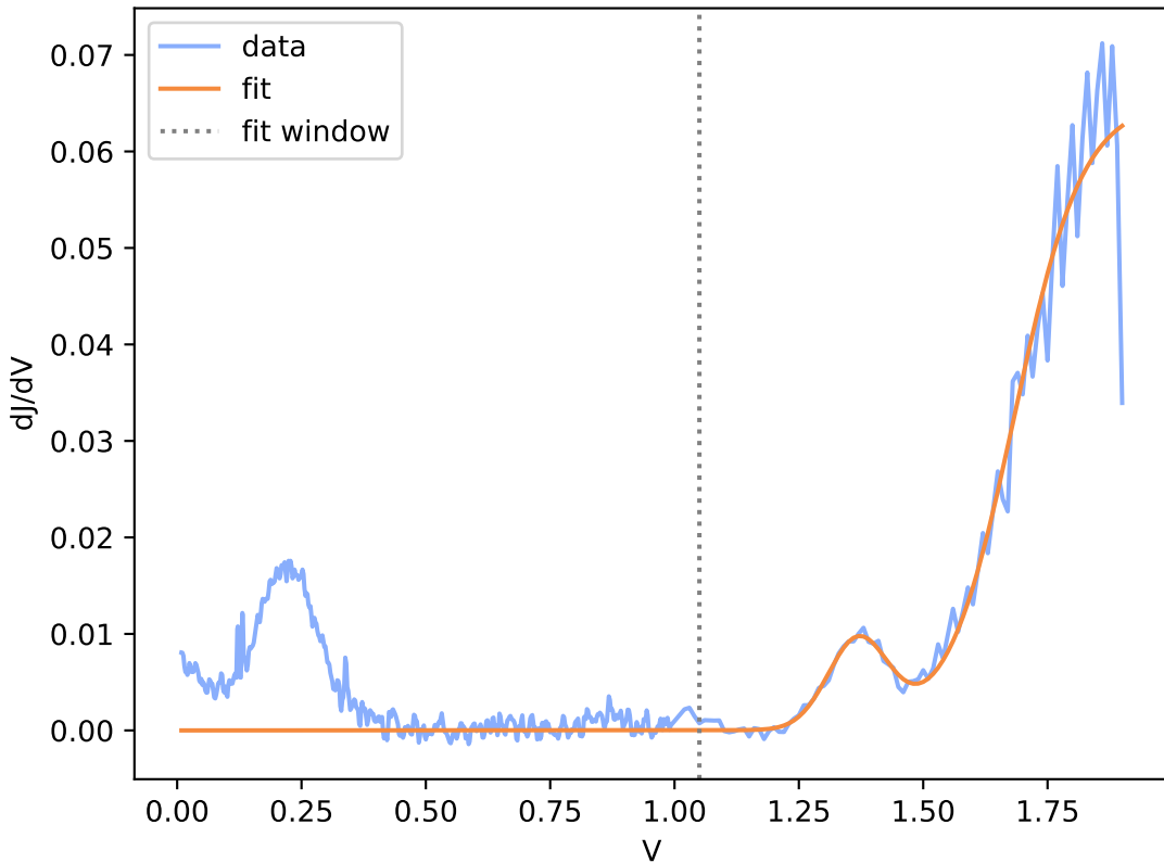
Run9-2-spot39.DTA.csv (window R^2 = 0.960 )
