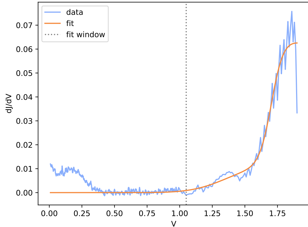
run11-2-spot2.DTA.csv (window R^2 = 0.954 )
