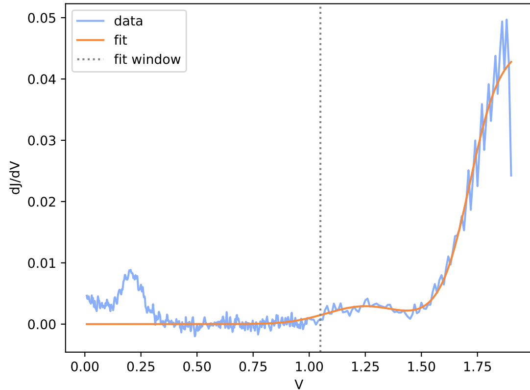
run11-2-spot21.DTA.csv (window R^2 = 0.957 )
