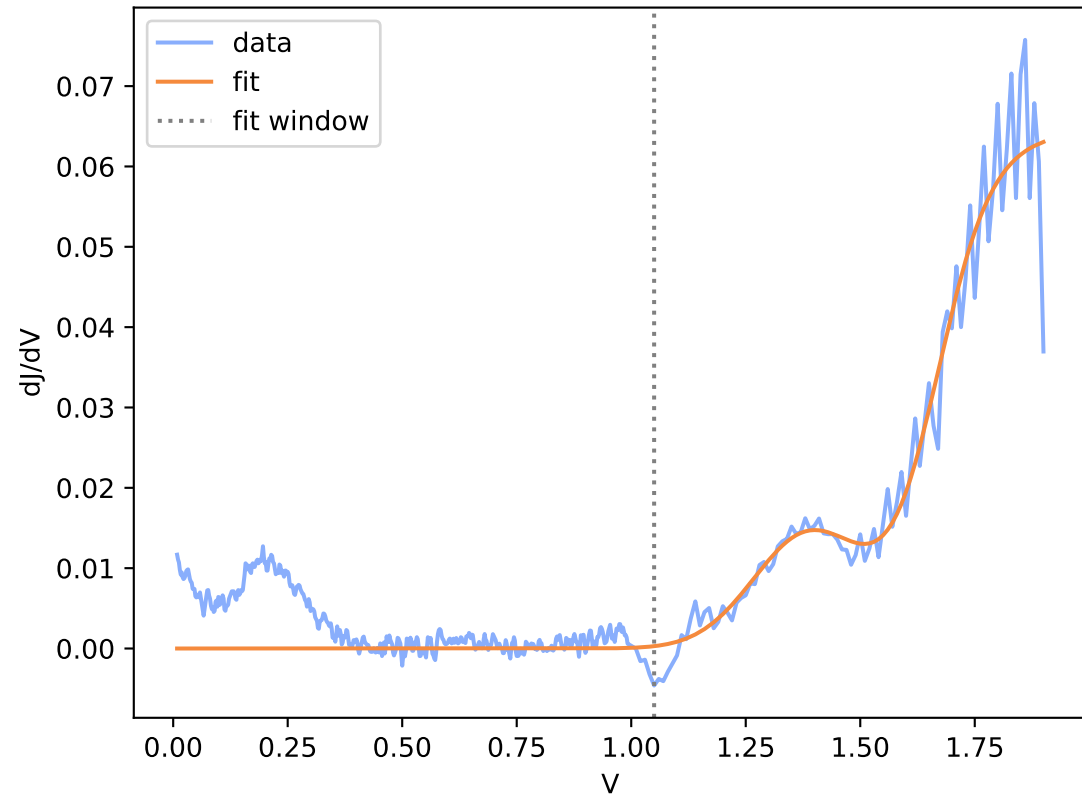
run9-2-spot10-2.DTA.csv (window R^2 = 0.950 )
