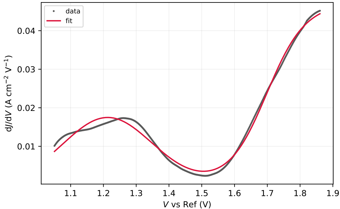
Run10-2-spot1.DTA.csv (window R^2 = 0.9913 )
