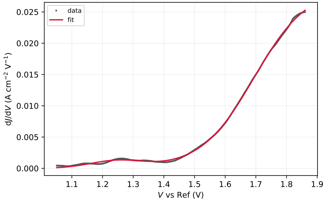
Run10-2-spot34.DTA.csv (window R^2 = 0.9996 )
