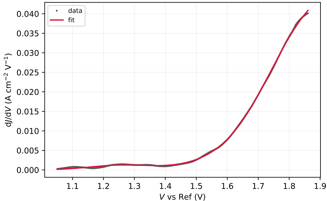
Run10-2-spot35.DTA.csv (window R^2 = 0.9997 )
