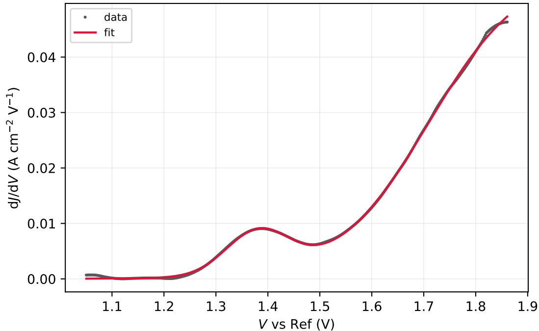
Run10-2-spot39.DTA.csv (window R^2 = 0.9997 )
