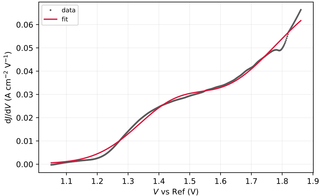
Run12-spot22.DTA.csv (window R^2 = 0.9943 )
