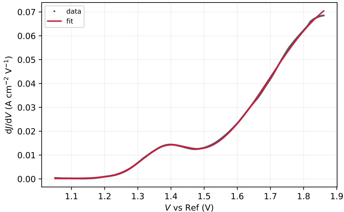
Run12-spot4.DTA.csv (window R^2 = 0.9997 )
