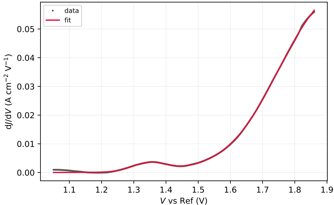
Run9-2-spot38.DTA.csv (window R^2 = 0.9997 )
