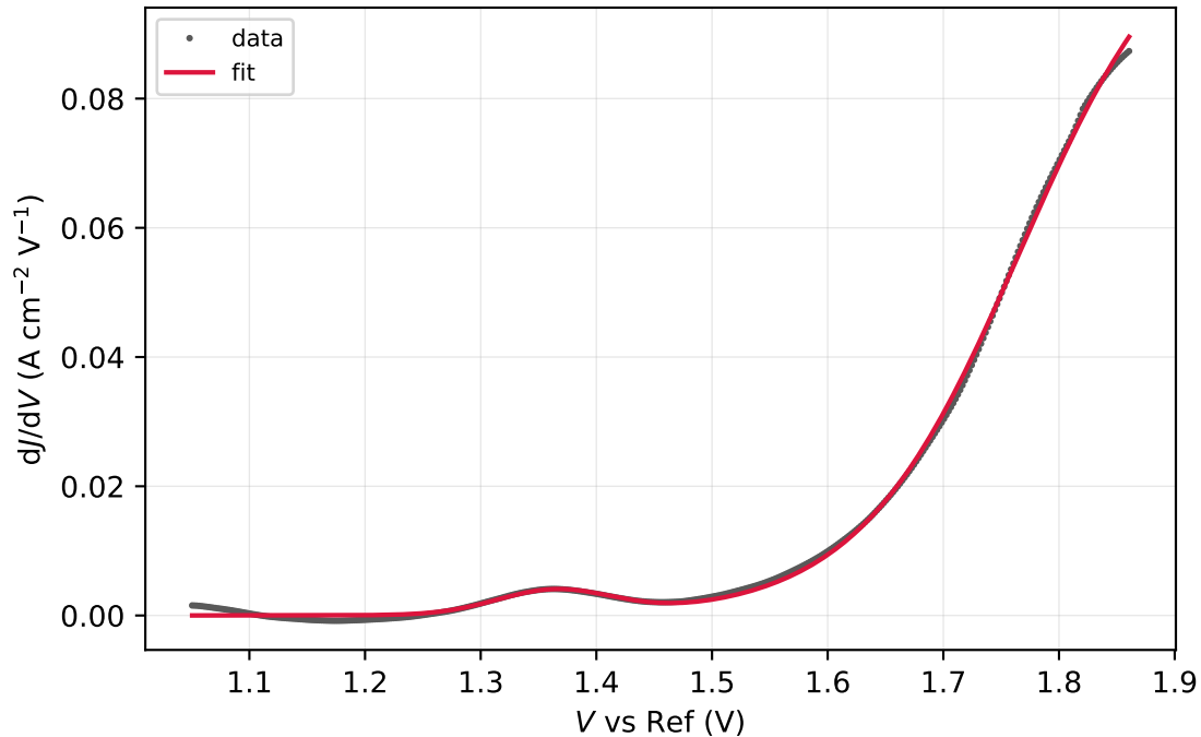
run11-2-spot30.DTA.csv (window R^2 = 0.9994 )
