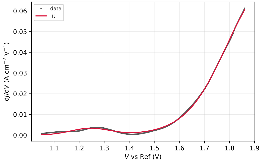
run11-2-spot34.DTA.csv (window R^2 = 0.9991 )
