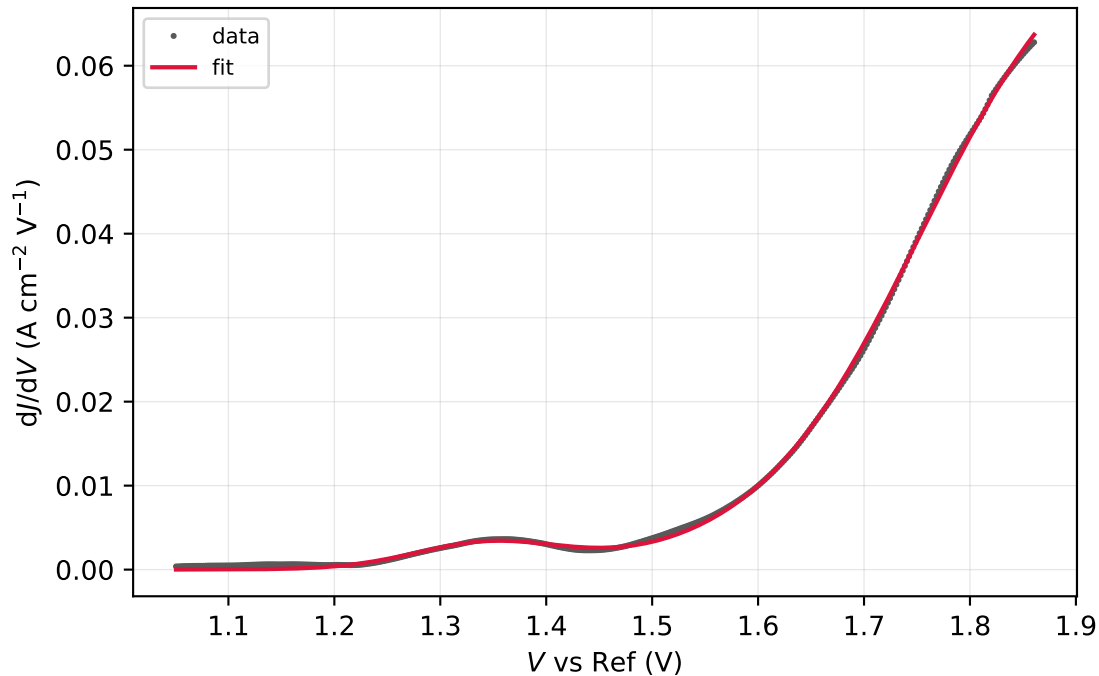
run11-2-spot7.DTA.csv (window R^2 = 0.9996 )
