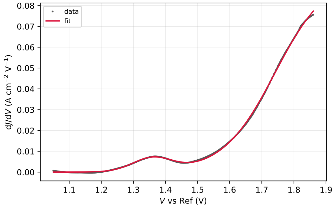
run11-2-spot8.DTA.csv (window R^2 = 0.9997 )
