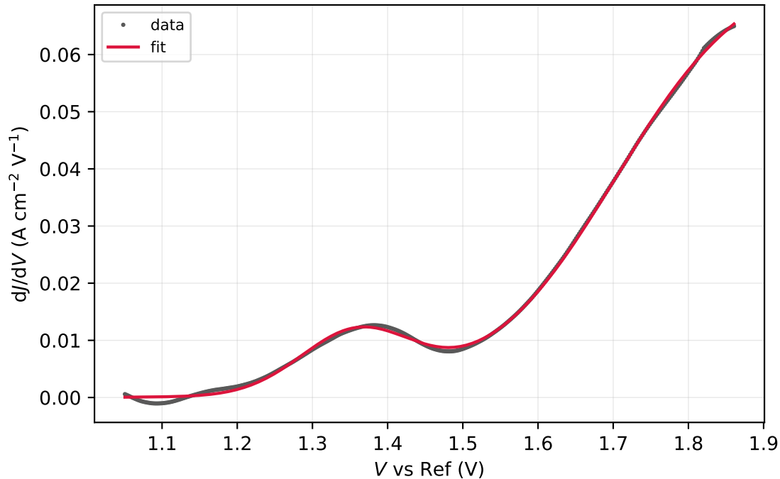
run9-2-spot17.DTA.csv (window R^2 = 0.9995 )
