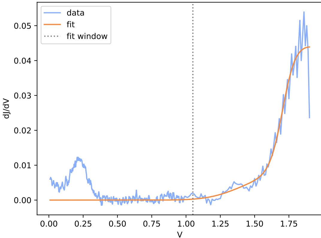
Run10-2-spot30.DTA.csv (window R^2 = 0.956 )
