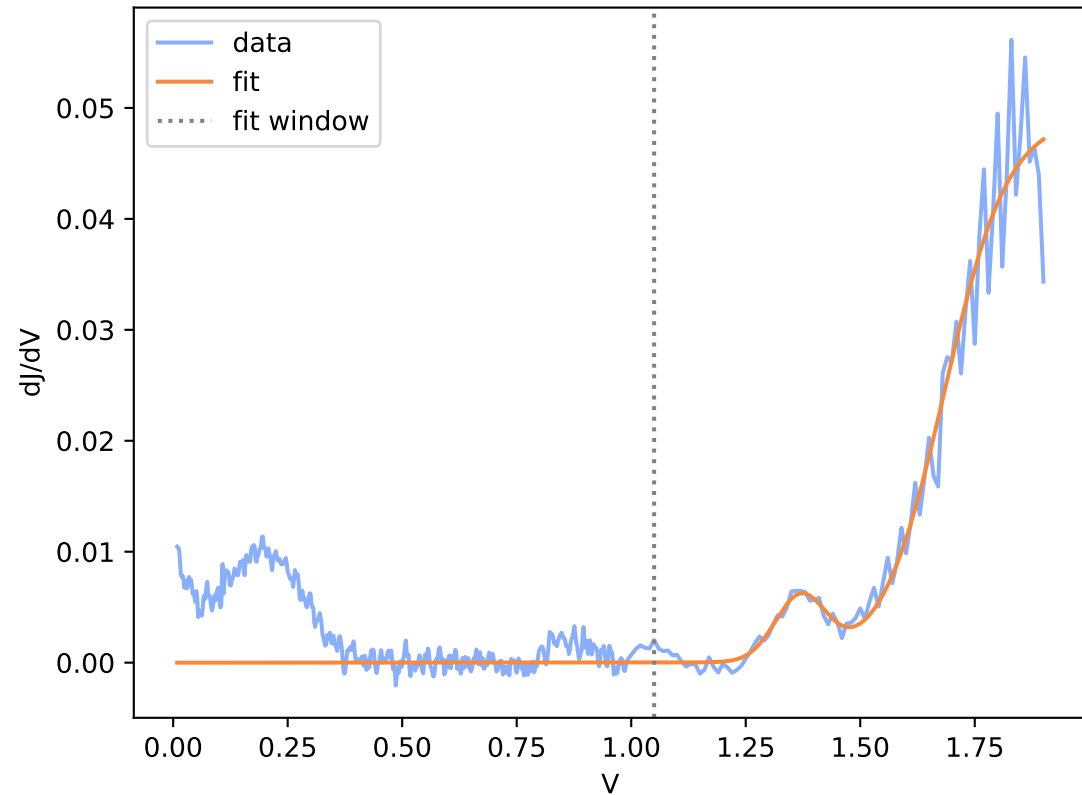
Run10-2-spot38.DTA.csv (window R^2 = 0.965 )
