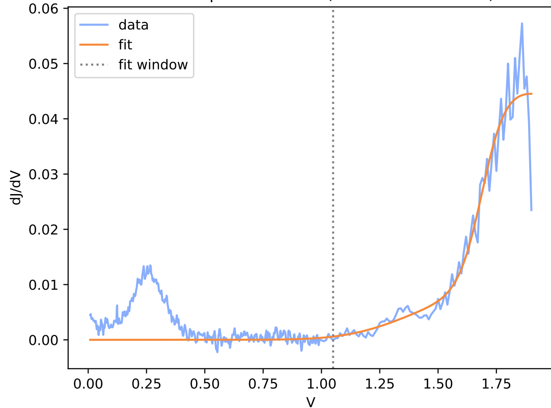
Run10-2-spot8.DTA.csv (window R^2 = 0.950 )
