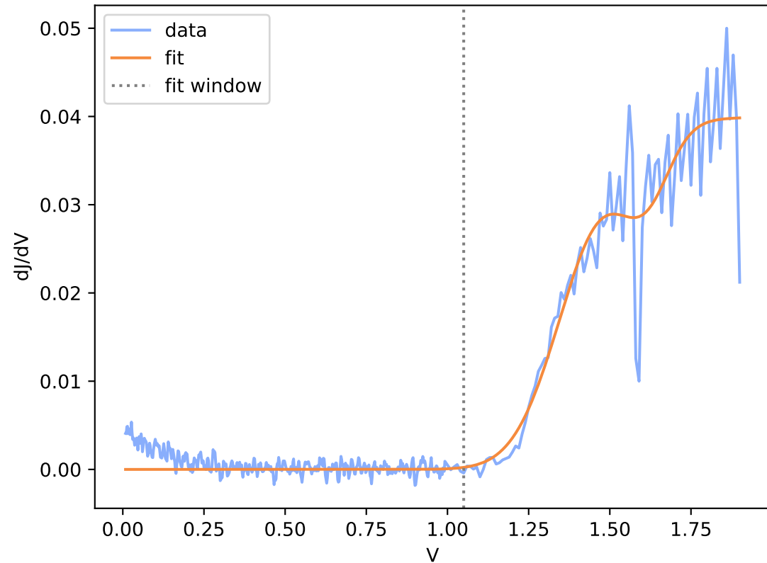
Run12-spot32.DTA.csv (window R^2 = 0.898 )
