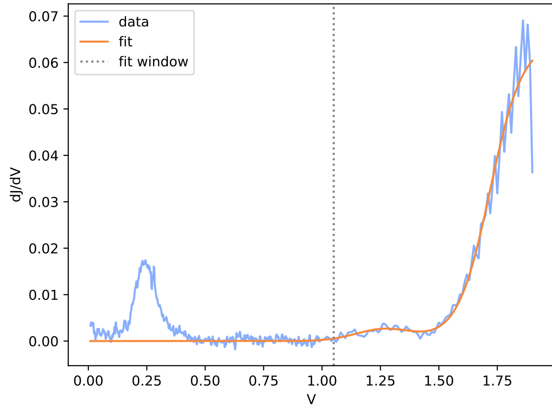
Run9-2-spot37.DTA.csv (window R^2 = 0.965 )
