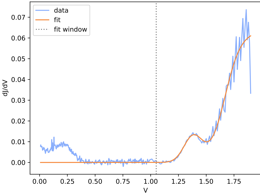
run9-2-spot25.DTA.csv (window R^2 = 0.950 )
