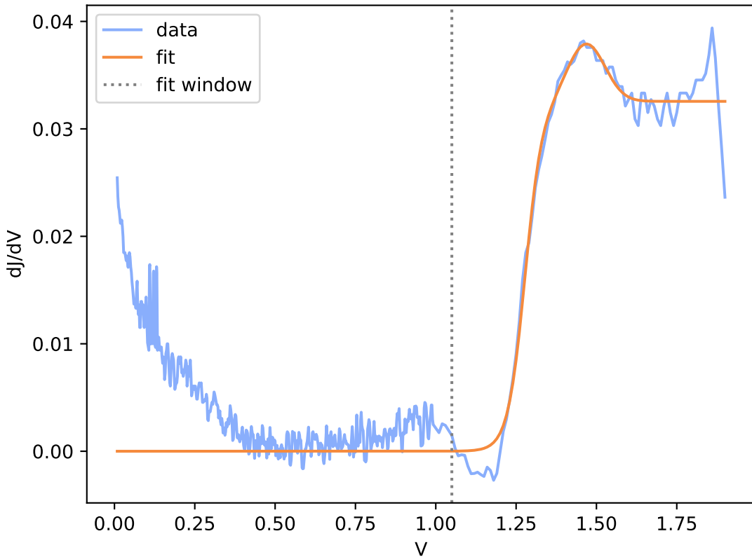
Run10-2-spot11.DTA.csv (window R^2 = 0.982 )
