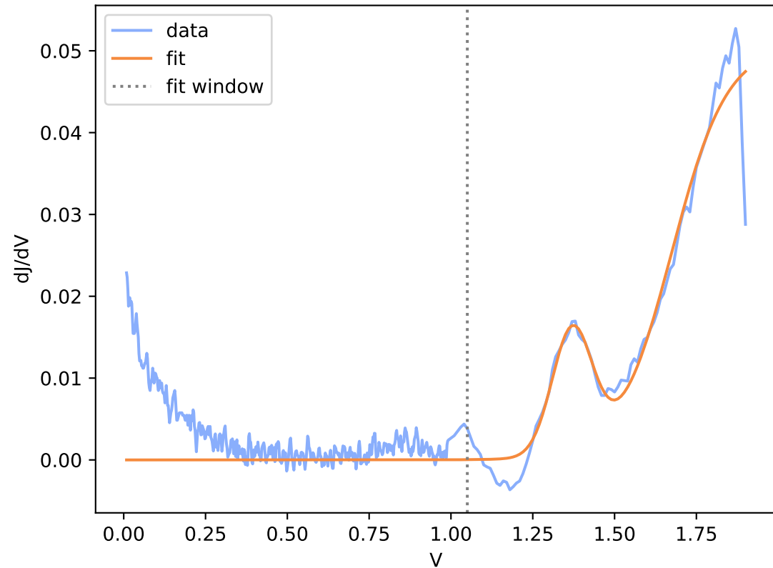
Run10-2-spot16.DTA.csv (window R^2 = 0.964 )
