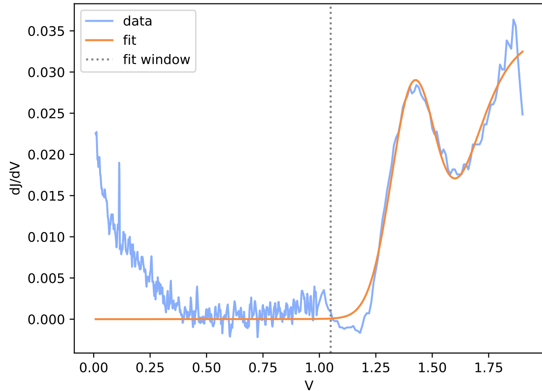
Run10-2-spot25.DTA.csv (window R^2 = 0.975 )
