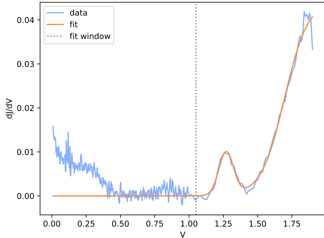
Run10-2-spot6.DTA.csv (window R^2 = 0.991 )
