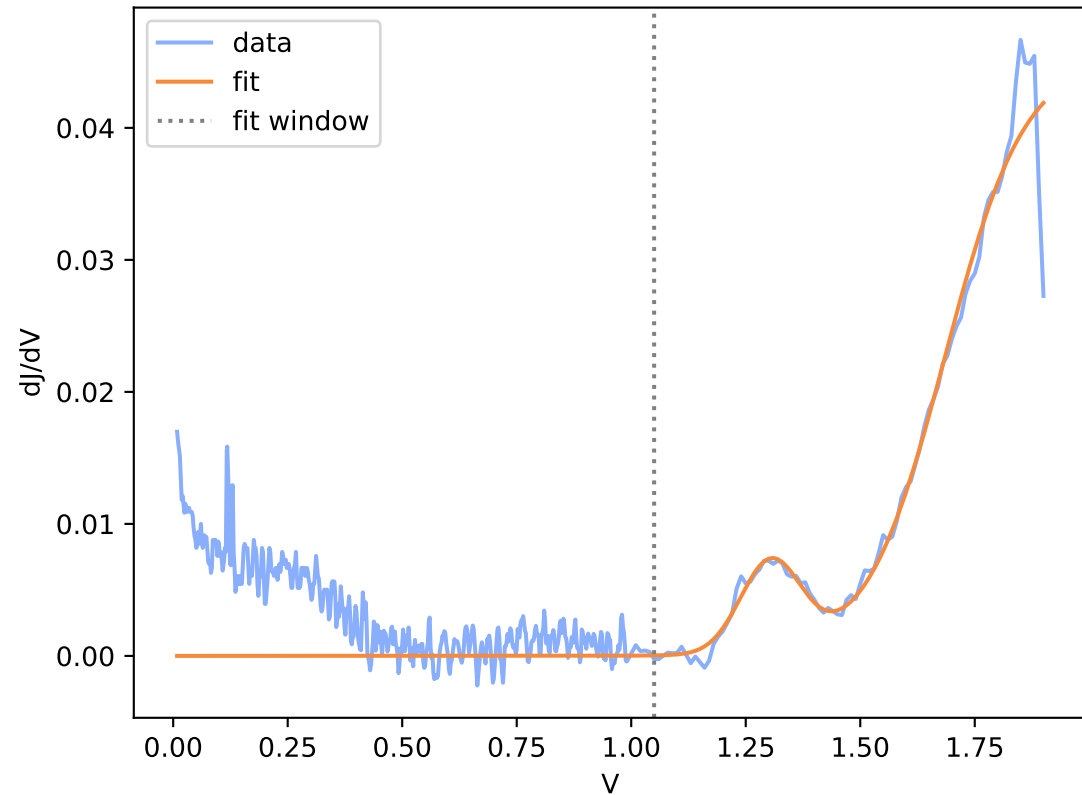
Run10-2-spot7.DTA.csv (window R^2 = 0.974 )
