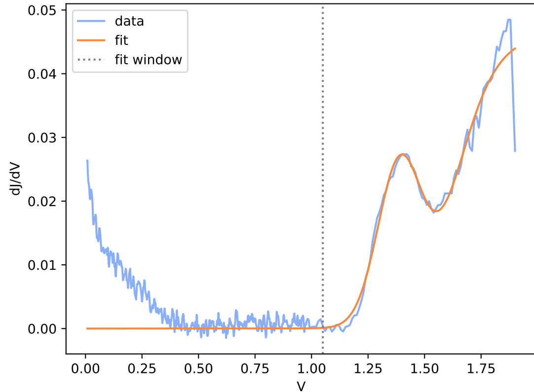
Run12-spot1.DTA.csv (window R^2 = 0.969 )
