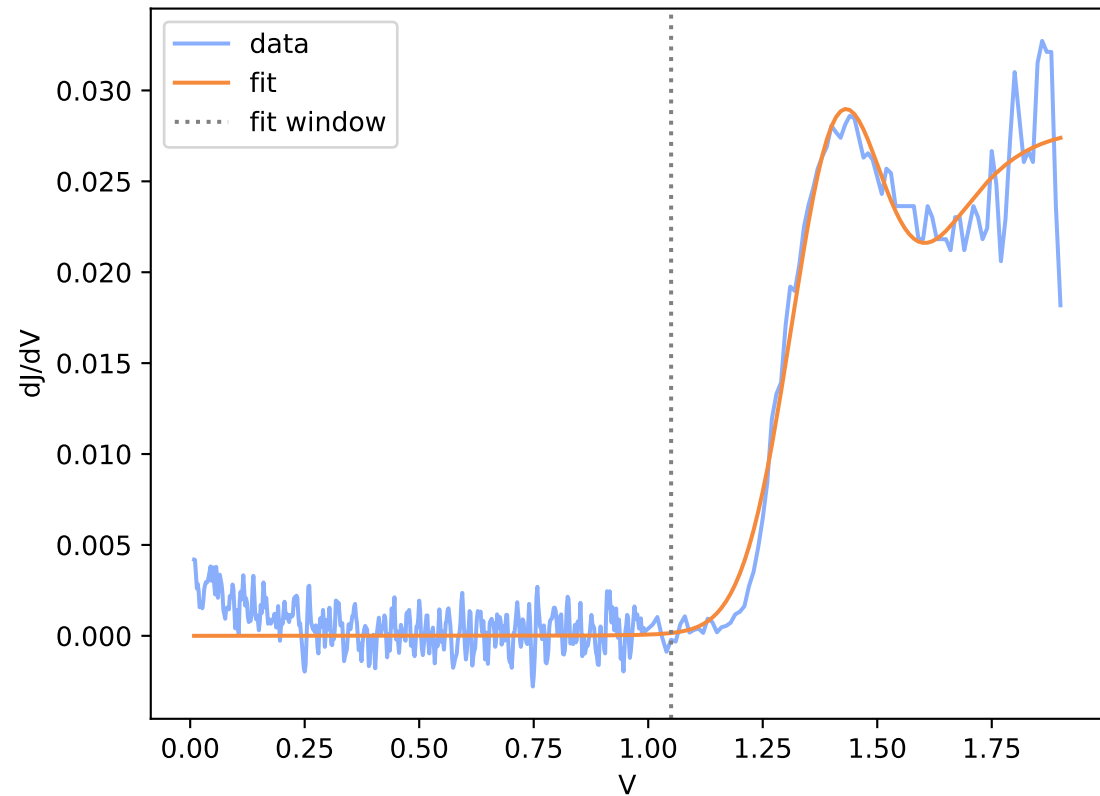
Run12-spot23.DTA.csv (window R^2 = 0.961 )
