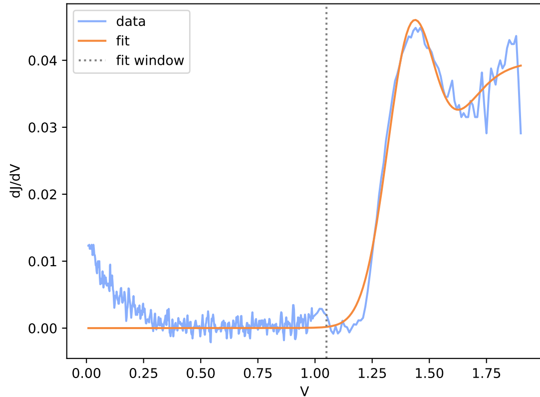
Run12-spot26.DTA.csv (window R^2 = 0.977 )
